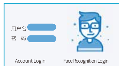
Login Method
